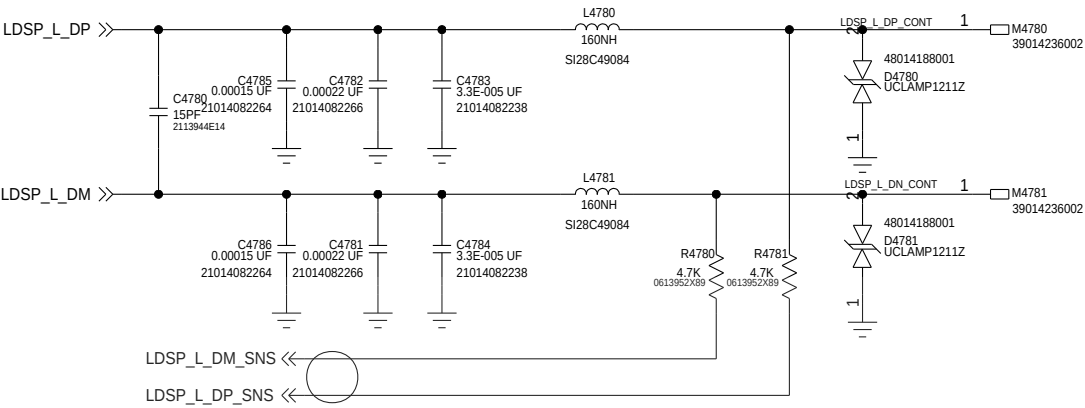
LOUDSPEAKER/EAR PIECE
